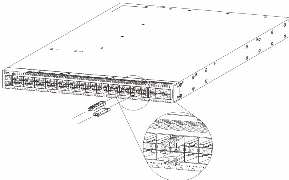
Figure 12. Inserting SFP/SFP+ transceivers into the SFP+ ports
