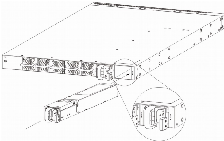
Figure 13. Installing an AC PSU Module
