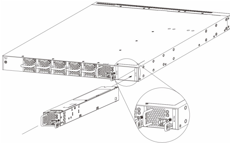
Figure 15. Installing a DC PSU Module
