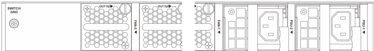
Figure 5. DXS-3610-54S Rear Panel LED Indicators
