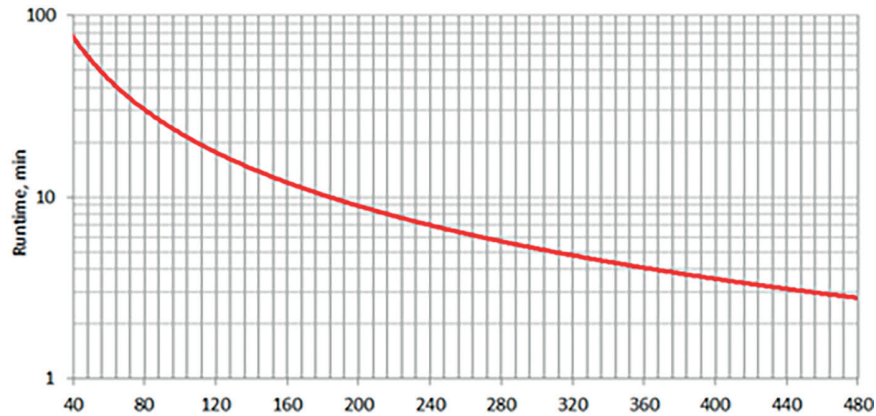
Figure 5. INFOPDU800 / INFOPDU800PL / INFOPDU800LCD autonomous operation schedule
