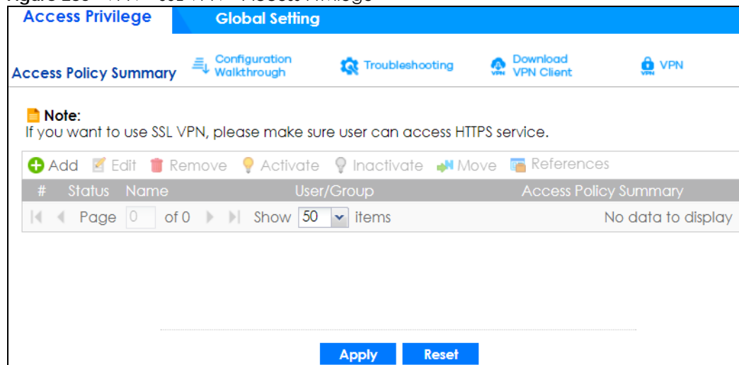
Figure 286 VPN > SSL VPN > Access Privilege
