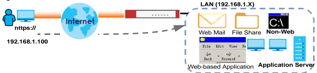
Figure 285 Network Access Mode: Full Tunnel Mode
