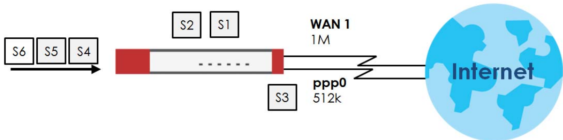
Figure 198 Weighted Round Robin Algorithm Example
